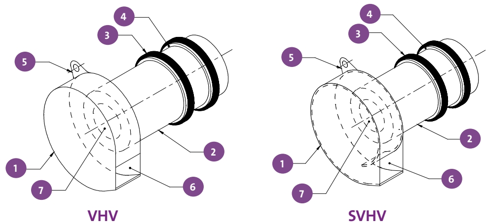
FIGURE 1: YDROVEX® VHV / SVHV VERTICAL VORTEX FLOW REGULATORS
